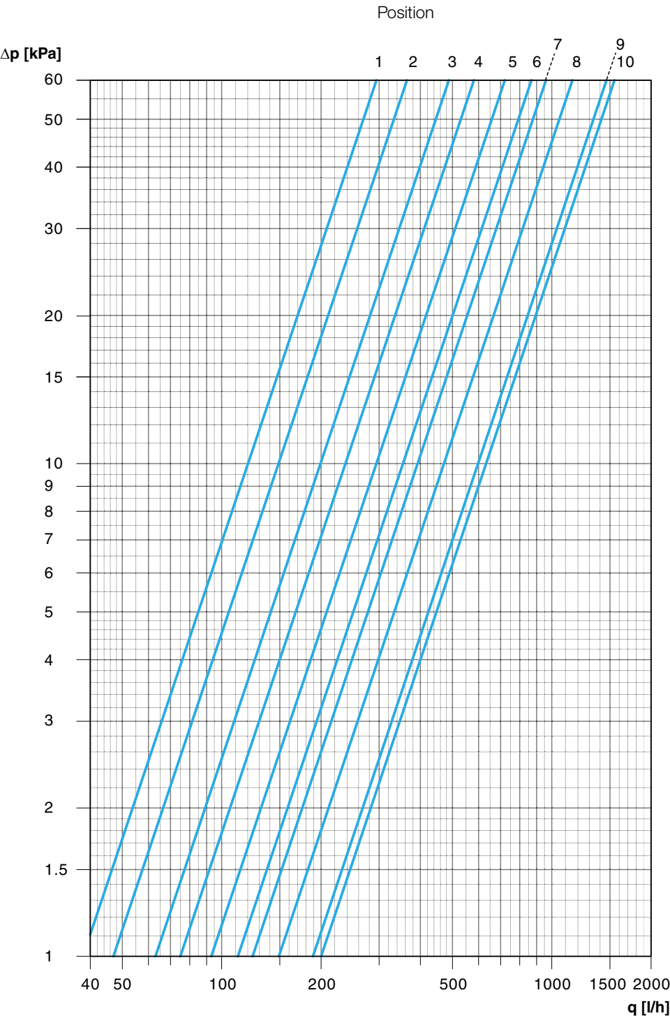
Diagram TBV-CM NF, DN 20
