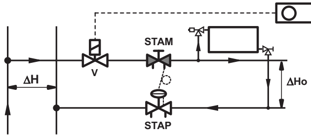
Fig 7.4c: The control valve is situated upstream the measuring valve STAM.
