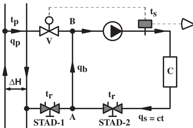
Fig. 8. Control of coil output for a coil supplied at constant flow.
