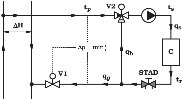
Fig. 18. Elimination of the primary differential pressure by means of a pressure controller.
