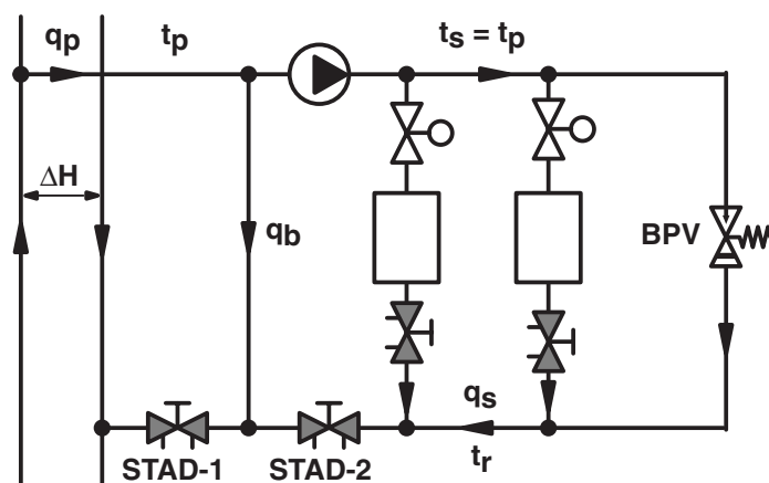
Fig. 13. Reducing or increasing the differential pressure applied across coils by means of a secondary pump.
