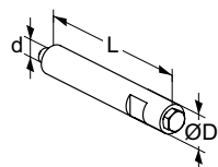
Venting extension Suitable when insulation is used. Stainless steel/EPDM/Brass.
