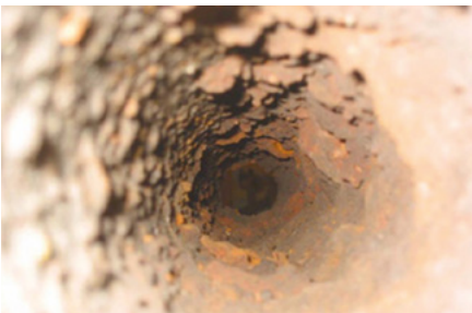
Internal view of 4» (DN 100) pipe due to corrosion
