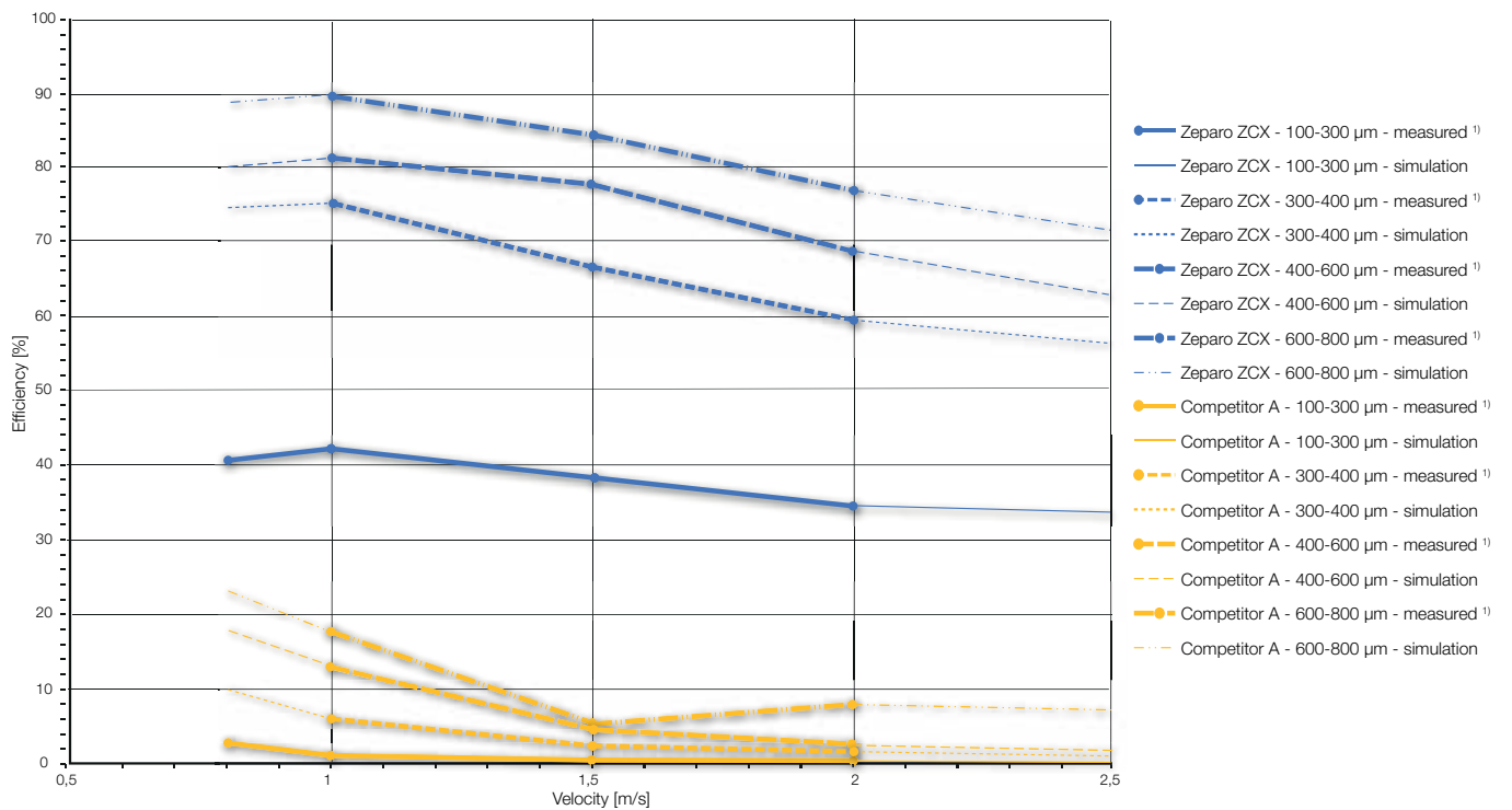
Separator DN200 - Glass particles with batch differentiation 100-800 \mu\text{m}
