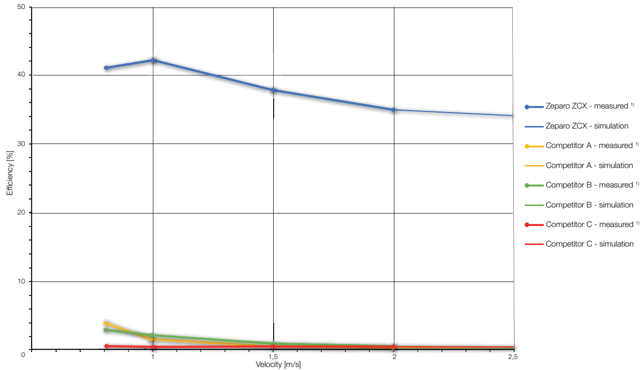
Separator DN200 - Glass particles 100-300 \mu\text{m}
