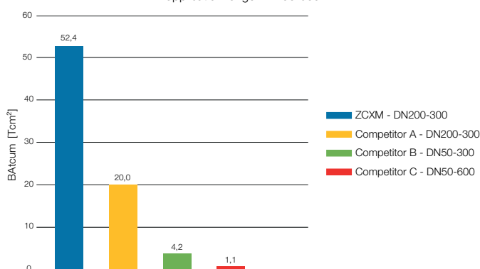
Cumulative magnetic flux over effective rod surface - application range DN200-300 2)
